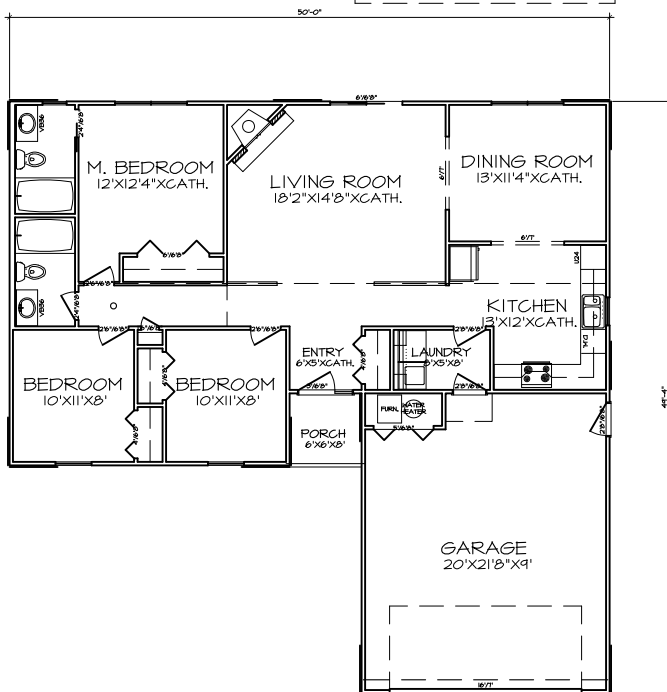
FIRST FLOOR PLAN A-4
